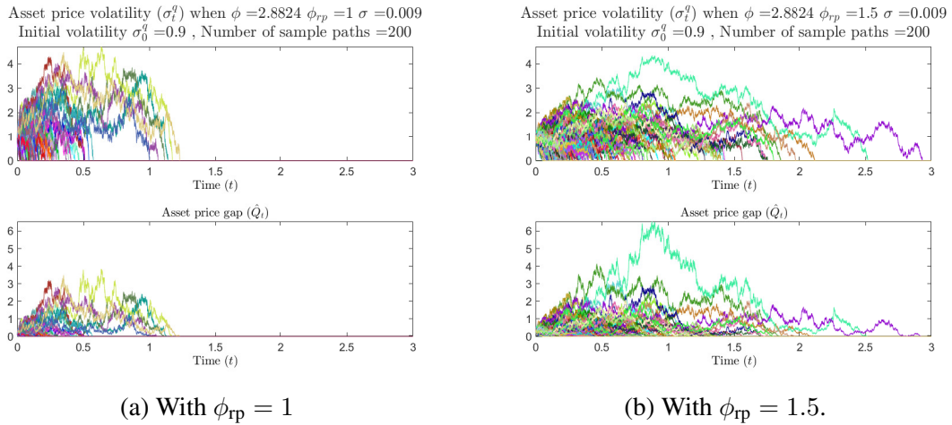
Figure D.7: \{\sigma_t^q, \hat{Q}_t\} dynamics when \sigma^{q,n} = 0 and \sigma_0^q = 0.9 , with varying \phi_{rp} > \frac{1}{2} .
